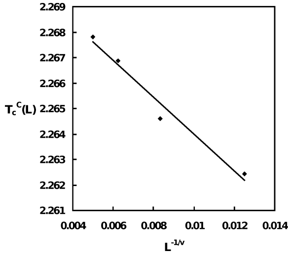
Fig. 3. The value of the infinite-lattice critical temperature for the specific heat C_L , T_c = 2.271(1) obtained by extrapolating the straight line fitted to critical temperatures of the lattice with linear dimensions 80 \leq L \leq 200 as L \rightarrow \infty .
