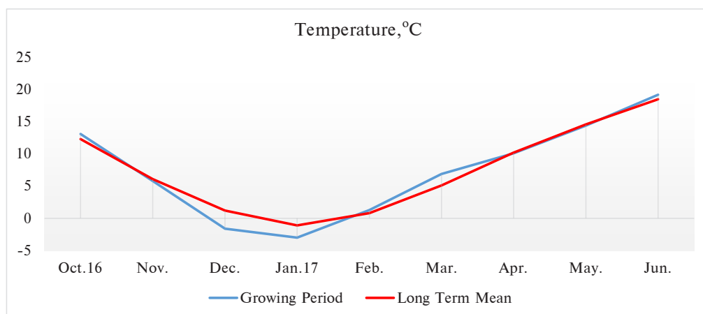
Figure 2. Monthly temperature values during the growing season (Turkish State Meteorological Service).
