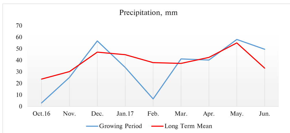
Figure 1. Monthly precipitation values during the growing season (Turkish State Meteorological Service).
