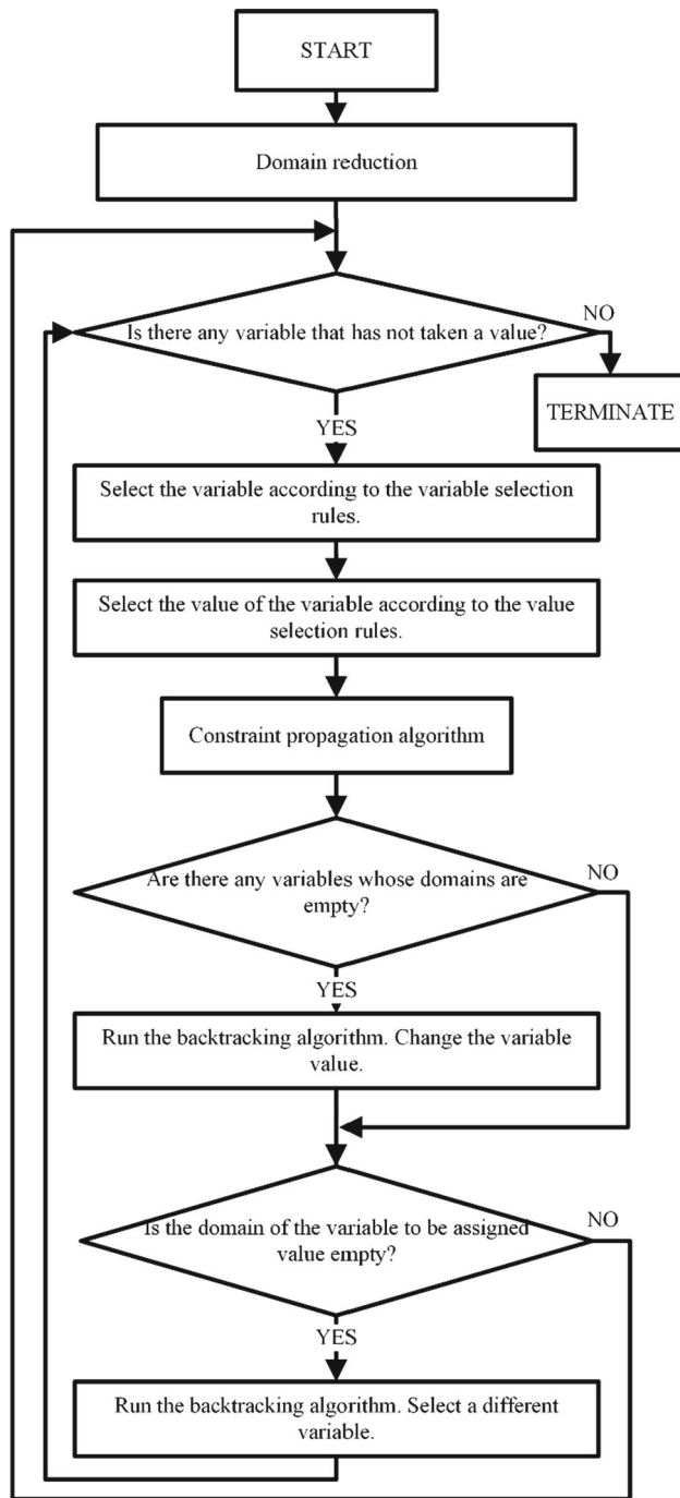
Fig. 1 Methodological flowchart of CP solution mechanism
