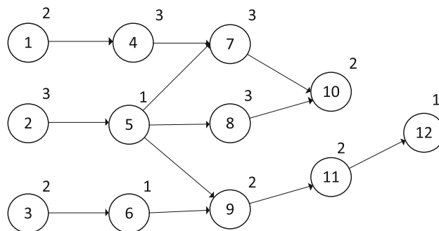
Fig. 2 Precedence diagram of the illustrative example
