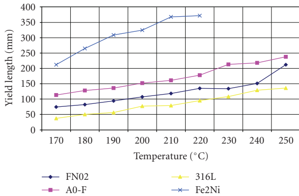
FIGURE 9: Yield length versus temperature graph for feedstocks.
