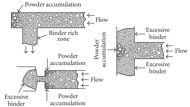
FIGURE 3: Separation of powder-binder during the direction change [2, 13].
