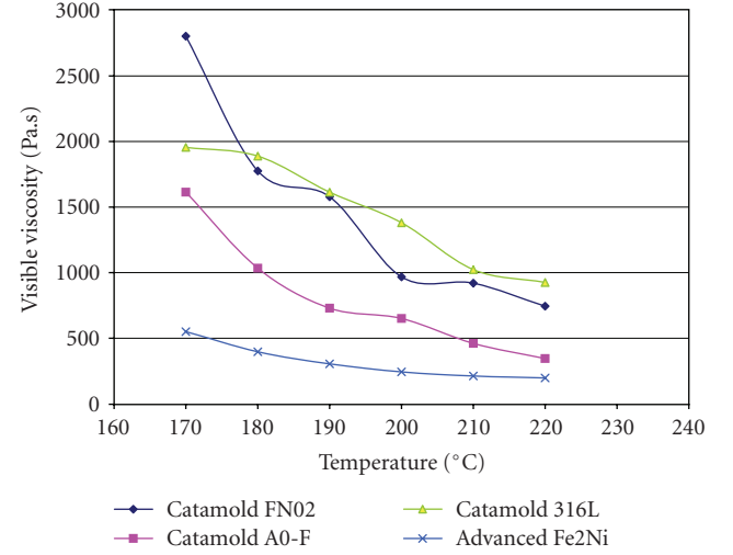
FIGURE 7: Temperature versus visible viscosity for present feedstocks (load 1,878 MPa).
