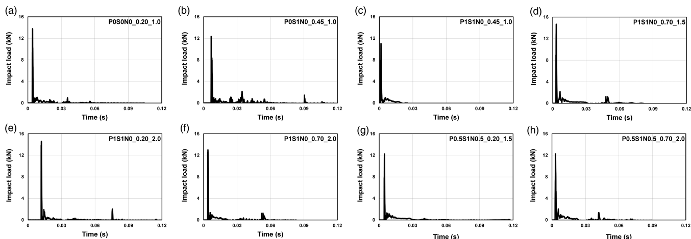
FIGURE 6 Representative impact load versus time graphs for selected specimens from different mixtures
