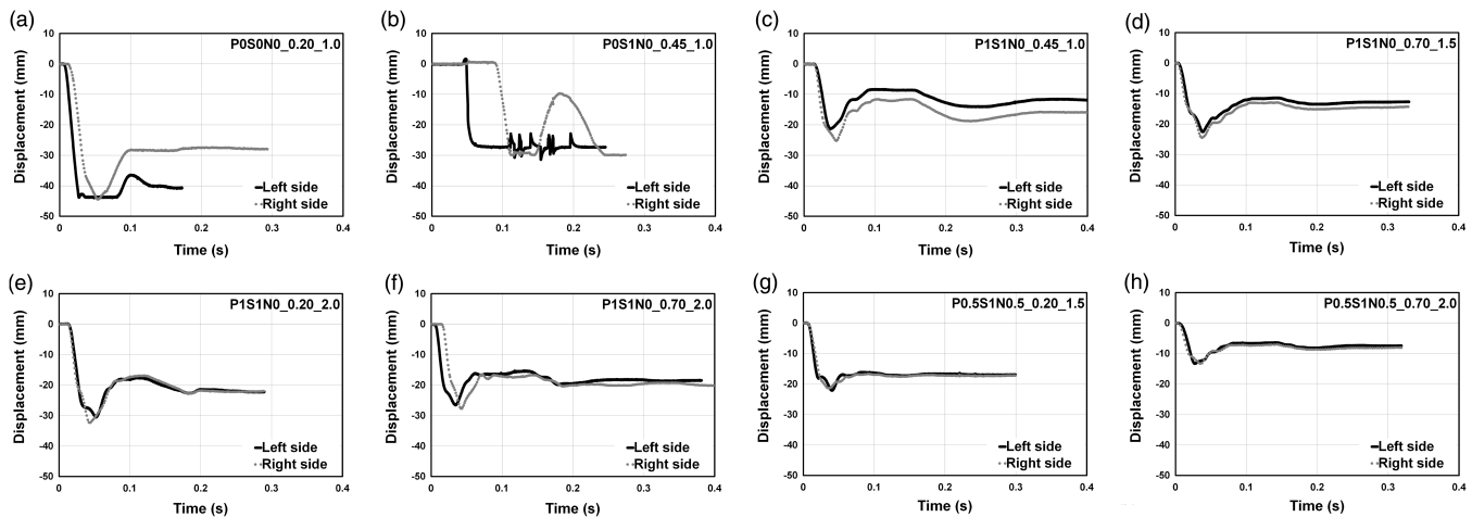
FIGURE 5 Representative displacement versus time graphs for selected specimens from different mixtures
