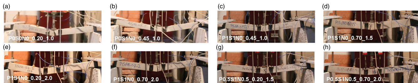
FIGURE 7 Representative views of the specimens from different mixtures after final failure
