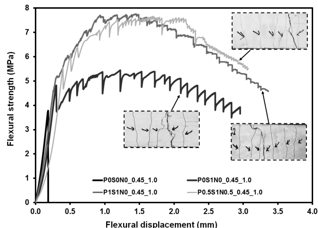
FIGURE 3 Effects of utilization of different types/dosages of fibers on typical flexural strength—displacement graphs and multiple microcracking behaviors of specimens
