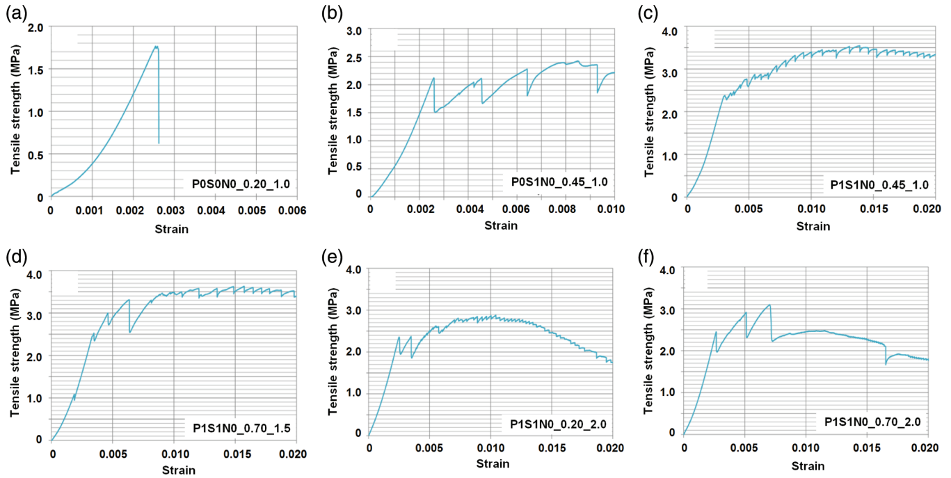
FIGURE 9 Representative uniaxial tensile stress versus strain models of specimens from different mixtures for FEA model
