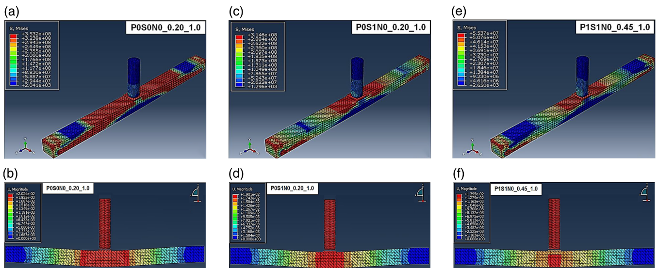
FIGURE 11 Representative stress distributions (a, c, e) and deformed shapes (b, d, f) of specimens from different mixtures during impact
