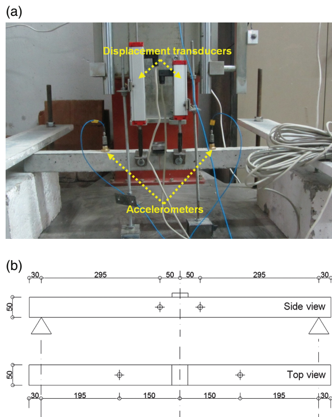
FIGURE 2 View of beam specimen ready for impact testing (a) and impact test layout (b) (all dimensions are in mm)
