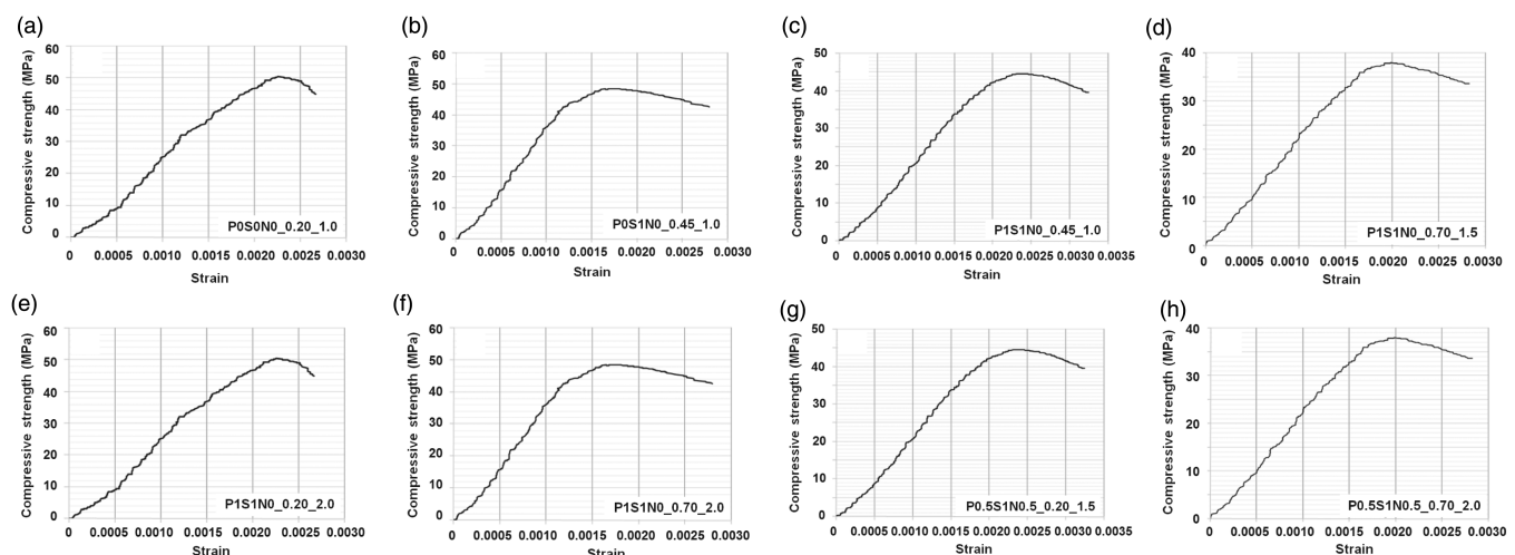
FIGURE 8 Representative compressive stress versus strain models of specimens from different mixtures for FEA model
