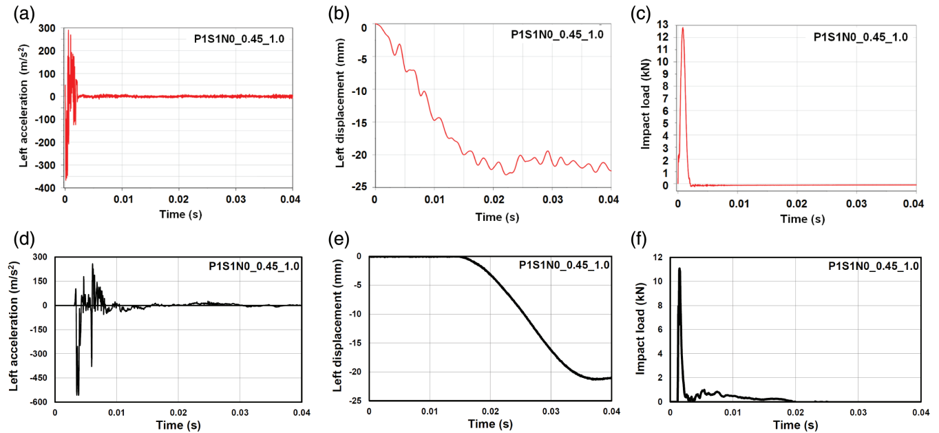
FIGURE 10 Acceleration versus time, displacement versus time, and impact load versus time graphs of specimens of P1S1N0_0.45_1.0 (Mixture #8) obtained from finite element analysis (a, b, c) and from real-time experiments (d, e, f)
