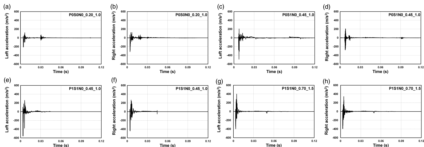
FIGURE 4 Representative acceleration versus time graphs for selected specimens from different mixtures
