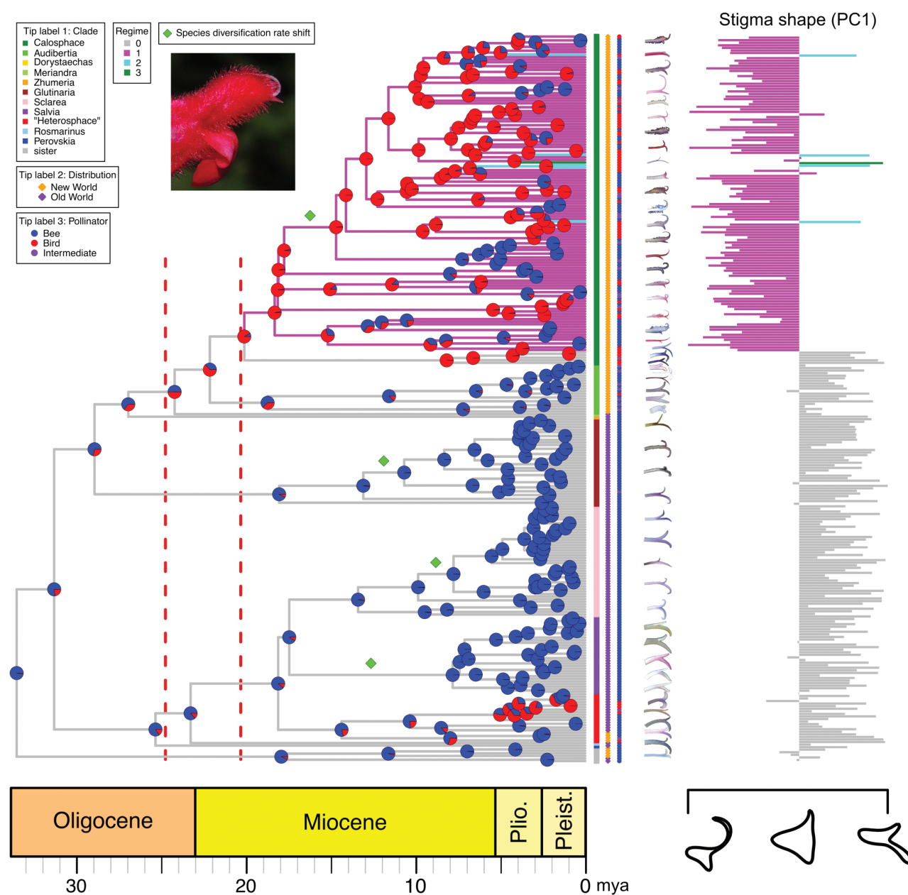
Figure 3. Univariate shift detection analysis with 11ou using PC1 from elliptic Fourier analysis of stigma shape in Salvia and close relatives. The left column depicts the phylogenetic tree with 263 tips based on the chronogram from Kriebel et al. (2019) with species dropped if not sampled. The four shifts in species diversification in Salvia from Kriebel et al. (2019) are indicated by green diamonds. Node pies represent the probability of each pollinator at each node. Tip labels (left to right) provide subgeneric placement and scoring for biogeographical area and pollinator. The right column depicts the score of PC1 for each tip (as a bar from the mean score) for stigma shape. Below the barplot a cartoon illustrates the mean (with its position indicated with a black dashed line) and the extreme shapes in PC1. Coloured PC1 lines (and the correspondent clade edges on the phylogenetic trees) represent separate regimes from the best shift configuration under the pBIC model selection criterion. Red dashed lines indicate ages of the stem and crown radiation of hummingbirds (McGuire et al. , 2014). The mouth of the corolla of hummingbird-pollinated Salvia oxyphora is shown to illustrate the curved stigma curving around the upper lip of the flower.
