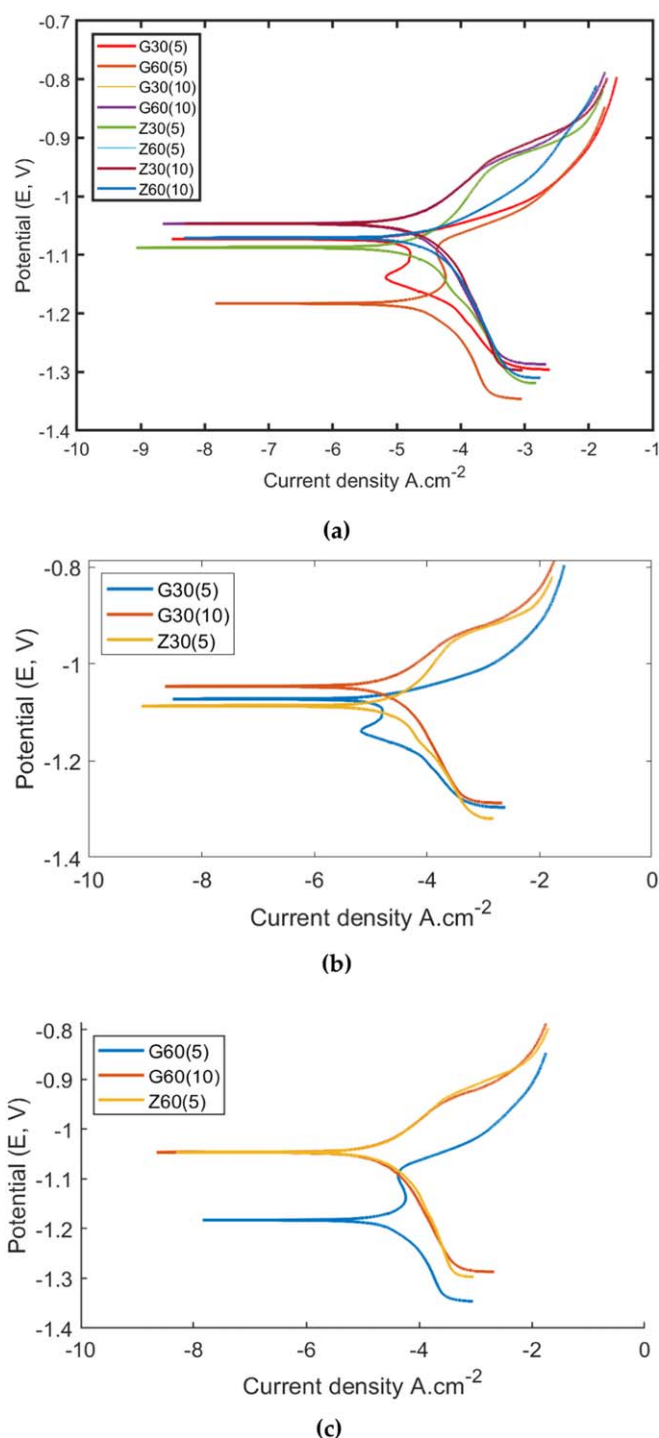
Figure 12. Potentiodynamic polarization curves (a) All samples, (b) samples G30-5, G30-10, Z30-5, (c) G60-5, G60-10, Z60-5.
