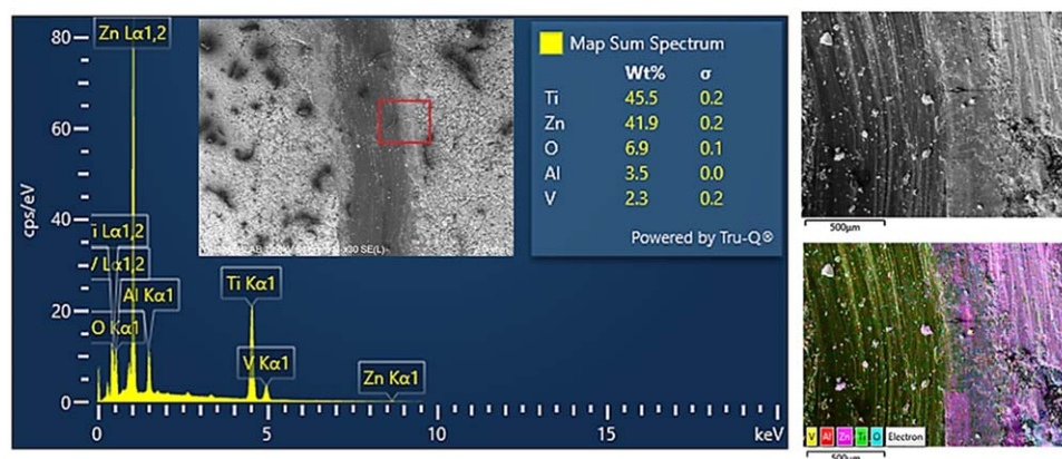
Figure 10. G30(10) wear path SEM and EDS examination.
