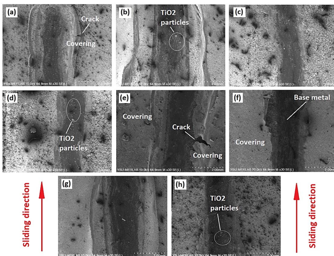
Figure 9. SEM images of wear path traces a) G30(5), b) G60(5), c) G30(10), d) G60(10), e) Z30(5), f) Z60(5), g) Z30(10) and h) Z60(10).
