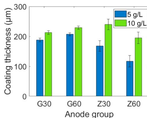
Figure 4. Average coating thickness values and cross-section image.
