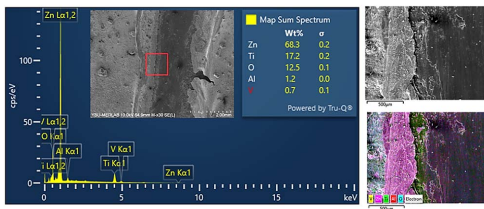
Figure 11. Z30(5) wear path SEM and EDS examination.
