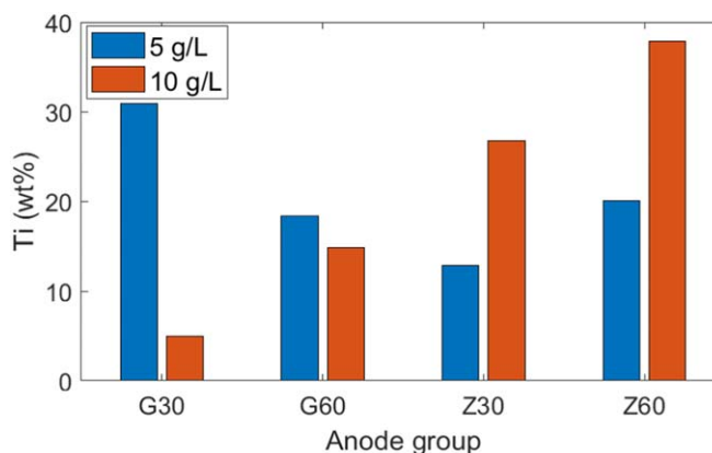
Figure 14. The EDS analysis results following the coating process indicate the weight percentage of Ti in the deposited coating on the surface.
