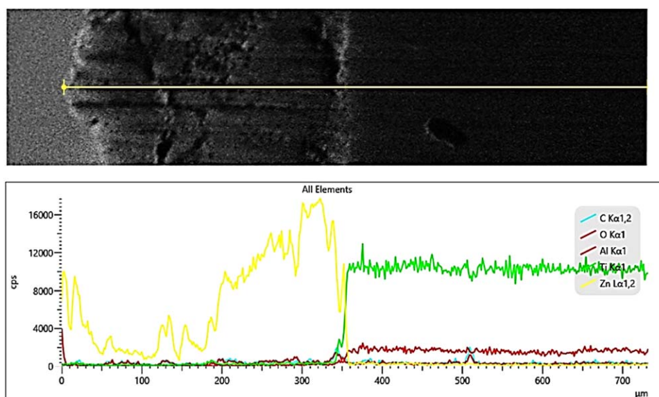
Figure 5. Cross-section EDS analysis example.
