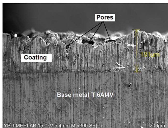
Figure 8. SEM image showing the microstructure of the coating region.
