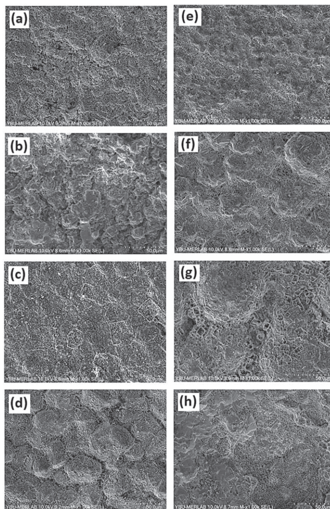
Figure 1. SEM images of Zn-doped \text{TiO}_2 coatings on Ti6Al4V alloy substrate produced using SLM (a) G30-5, (b) G60-5, (c) G30-10, (d) G60-10, (e) Z30-5, (f) Z60-5, (g) Z30-10, (h) Z60-10.
