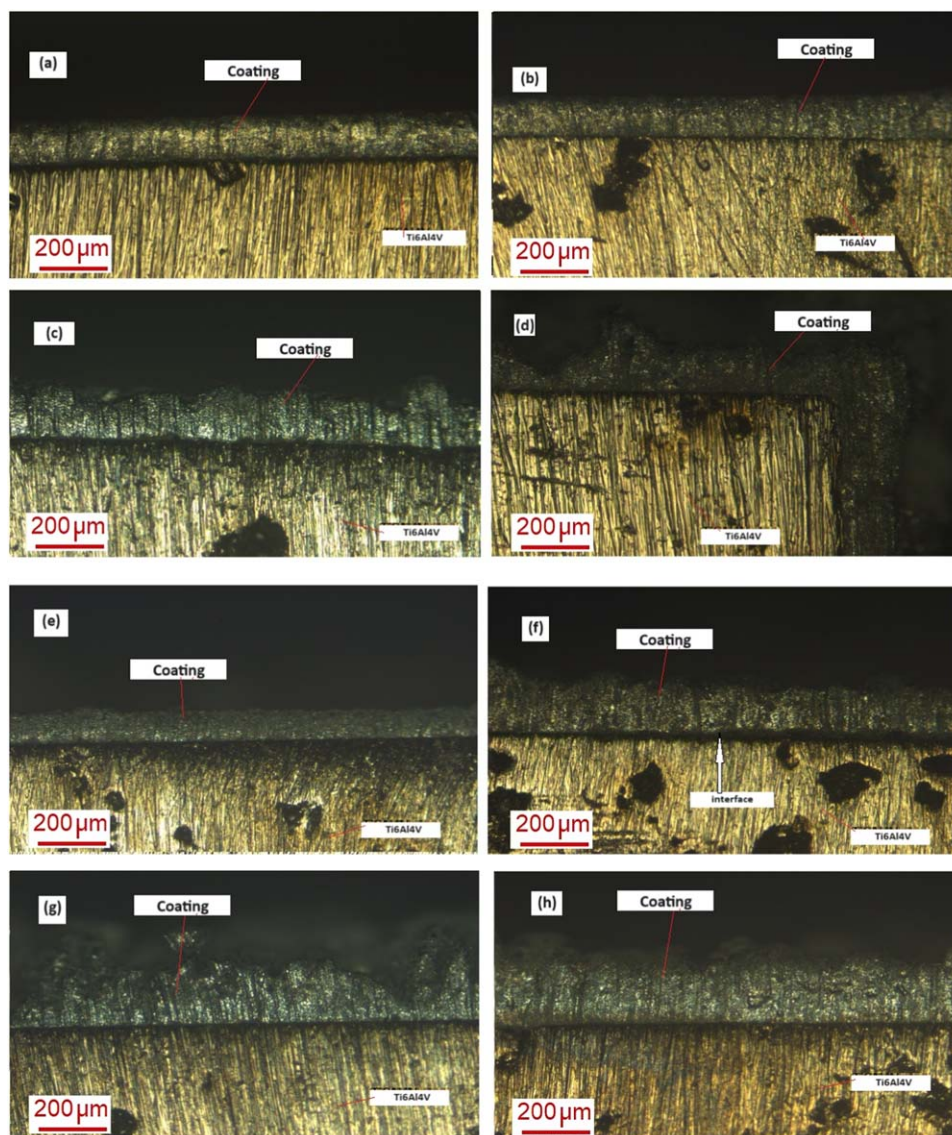
Figure 3. Optical microscope images of coating thicknesses (a) G30-5, (b) G60-5, (c) G30-10, (d) G60-10, (e) Z30-5, (f) Z60-5, (g) Z30-10, (h) Z60-10.
