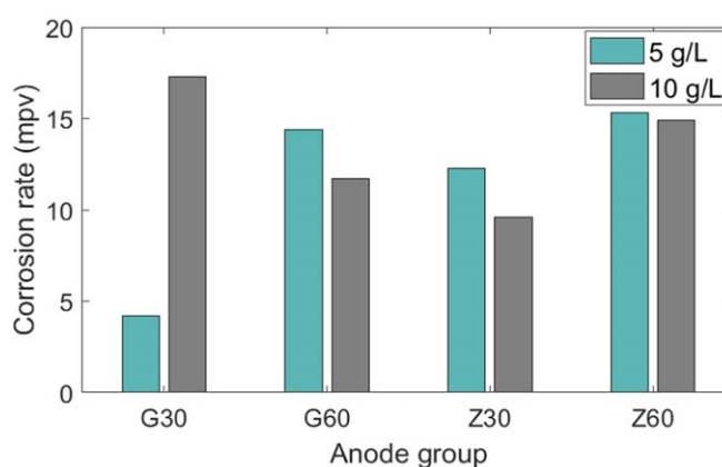
Figure 15. The variation in corrosion rate concerning the amount of TiO 2 addition.
