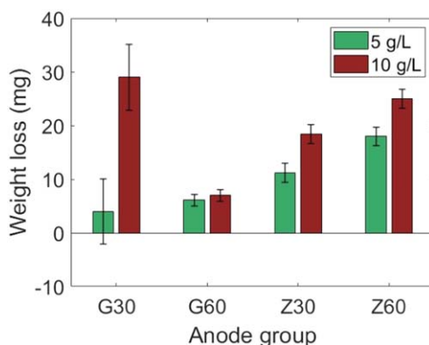
Figure 7. Wear loss change according to TiO 2 addition amount.
