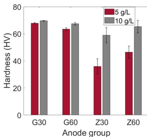
Figure 6. Hardness change according to TiO 2 addition amount.
