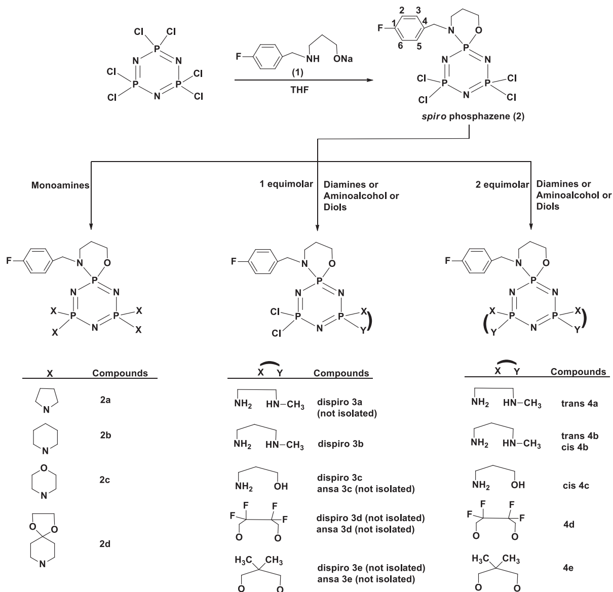
Scheme. The fully and partly substituted 4-fluorobenzylspirocyclotriphosphazenes.
