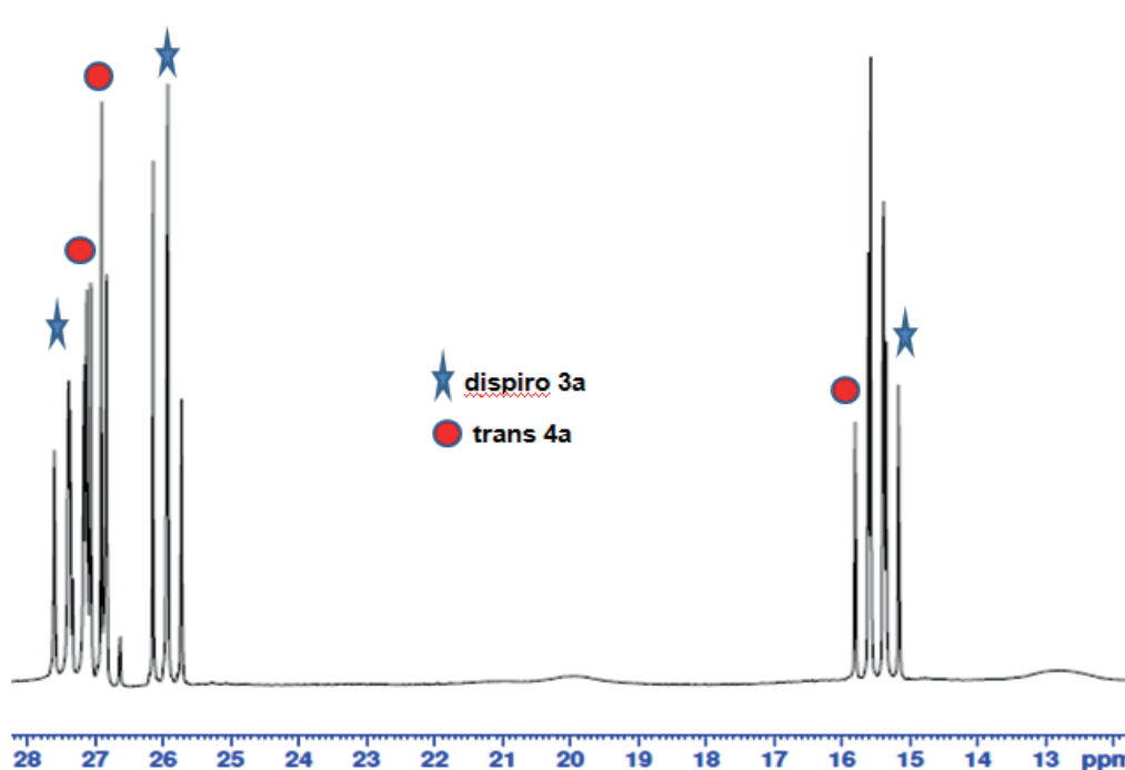
Figure 1. The ^{31}\text{P}\{^1\text{H}\} spectrum of the mixture of 2 and one equimolar amount of N-methylethylenediamine.
