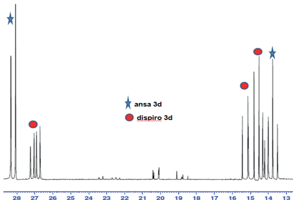
Figure 3. The ^{31}\text{P}\{^1\text{H}\} spectrum of the mixture of 2 and one equimolar amount of sodium 2,2,3,3-tetrafluorobutanedioide.
