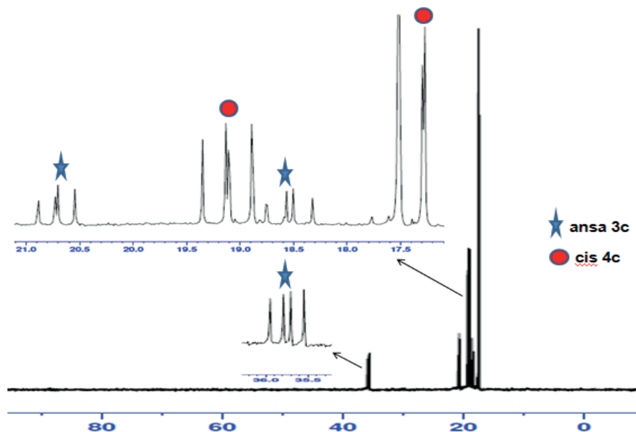
Figure 2. The ^{31}\text{P}\{^1\text{H}\} spectrum of the mixture of 2 and one equimolar amount of sodium 3-amino-1-propanoxide.
