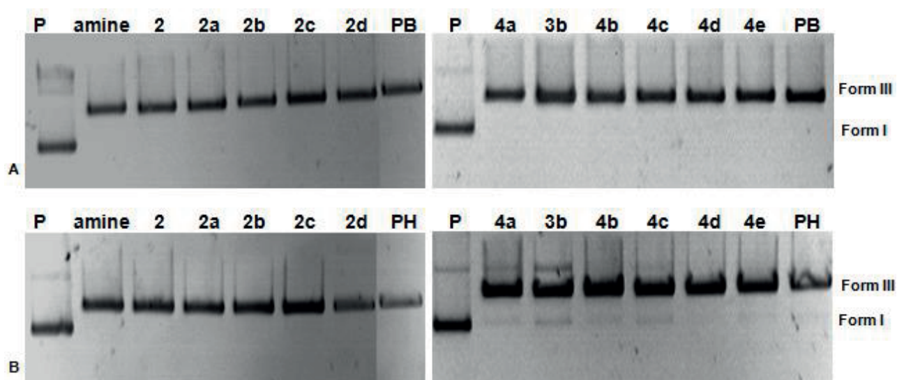
Figure 6. The electrophoretograms for A) Bam HI and B) Hind III digested mixtures of pBR322 DNA after treatment with the phosphazenes. Lane P is untreated plasmid DNA and lanes PH and PB are Hind III and Bam HI digestion of untreated DNA. The numbers above the lines indicate the compounds digested with the enzymes.
