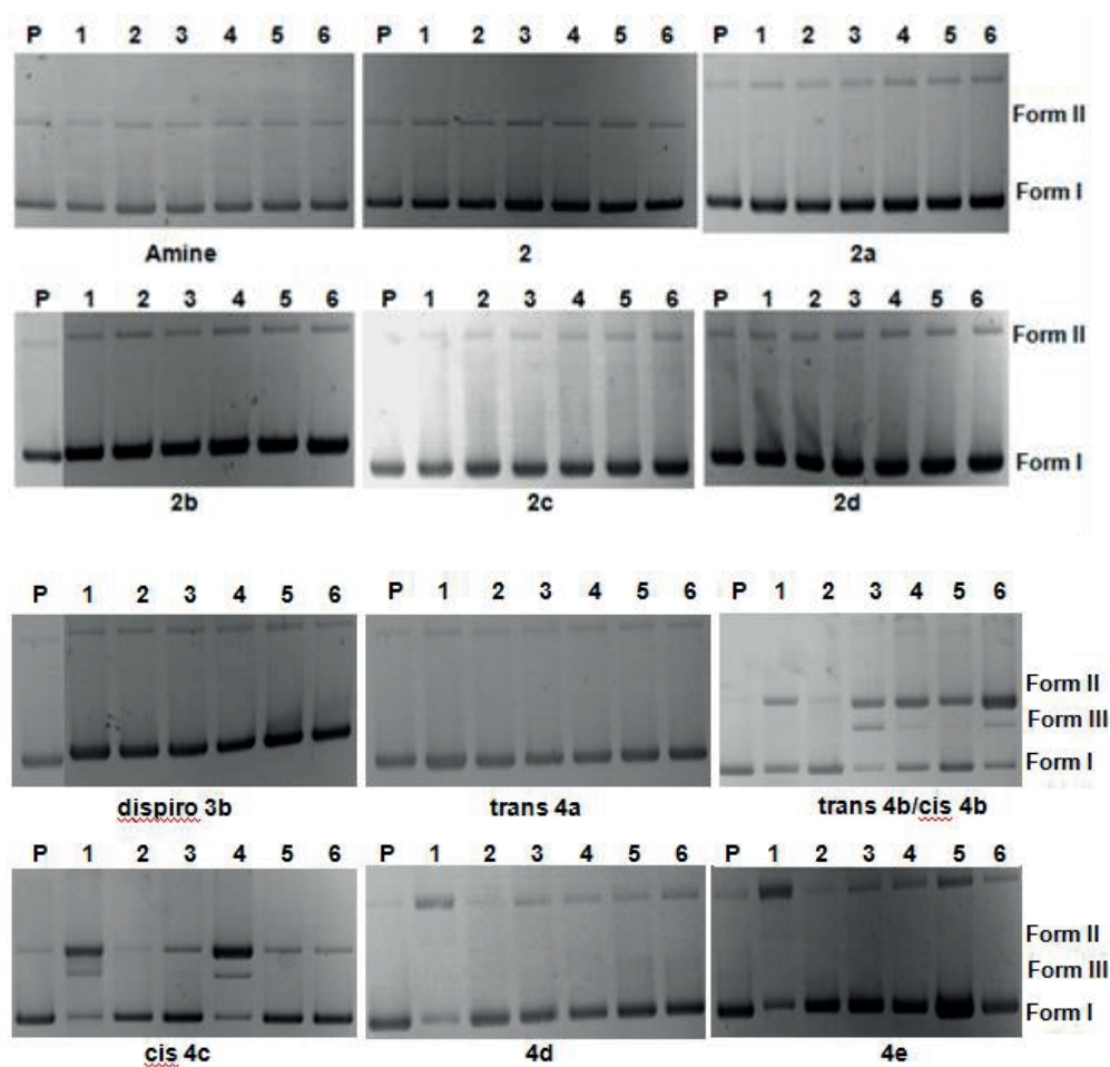
Figure 5. Gel electrophoretic mobilities of pBR322 DNA after incubation at concentrations ranging from 2500 to 78 \mu M at 37 °C. Line 1: 2500, line 2: 1250, line 3: 625, line 4: 312.50, line 5: 156.25, line 6: 78 ( \mu M), P: untreated plasmid.
