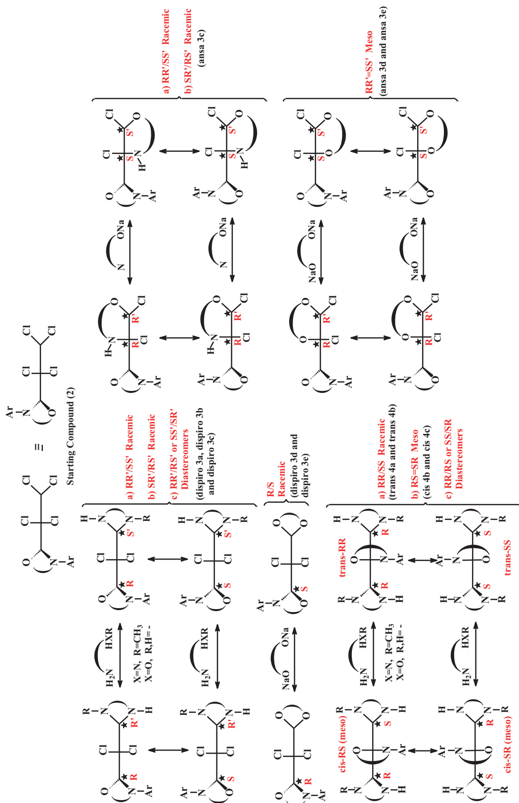
Figure 4. The expected and obtained isomer distributions of the partly and fully substituted phosphazene derivatives.
