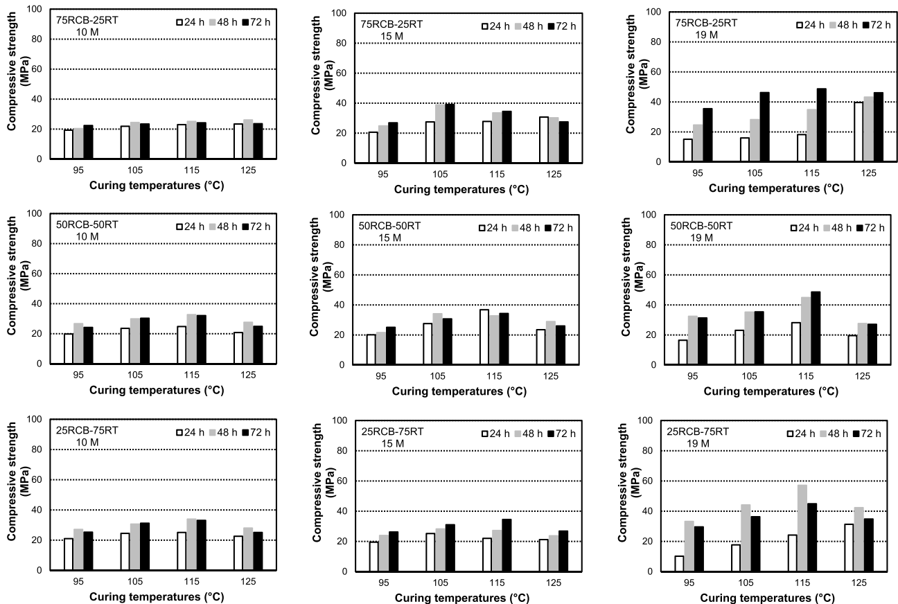
Fig. 4. Average compressive strength results of alkali-activated binders with different substitution rates of RCB and RT.
