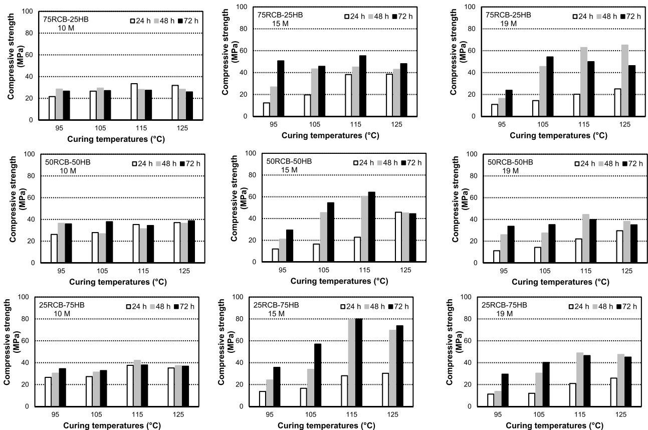
Fig. 5. Average compressive strength results of alkali-activated binders with different substitution rates of RCB and HB.
