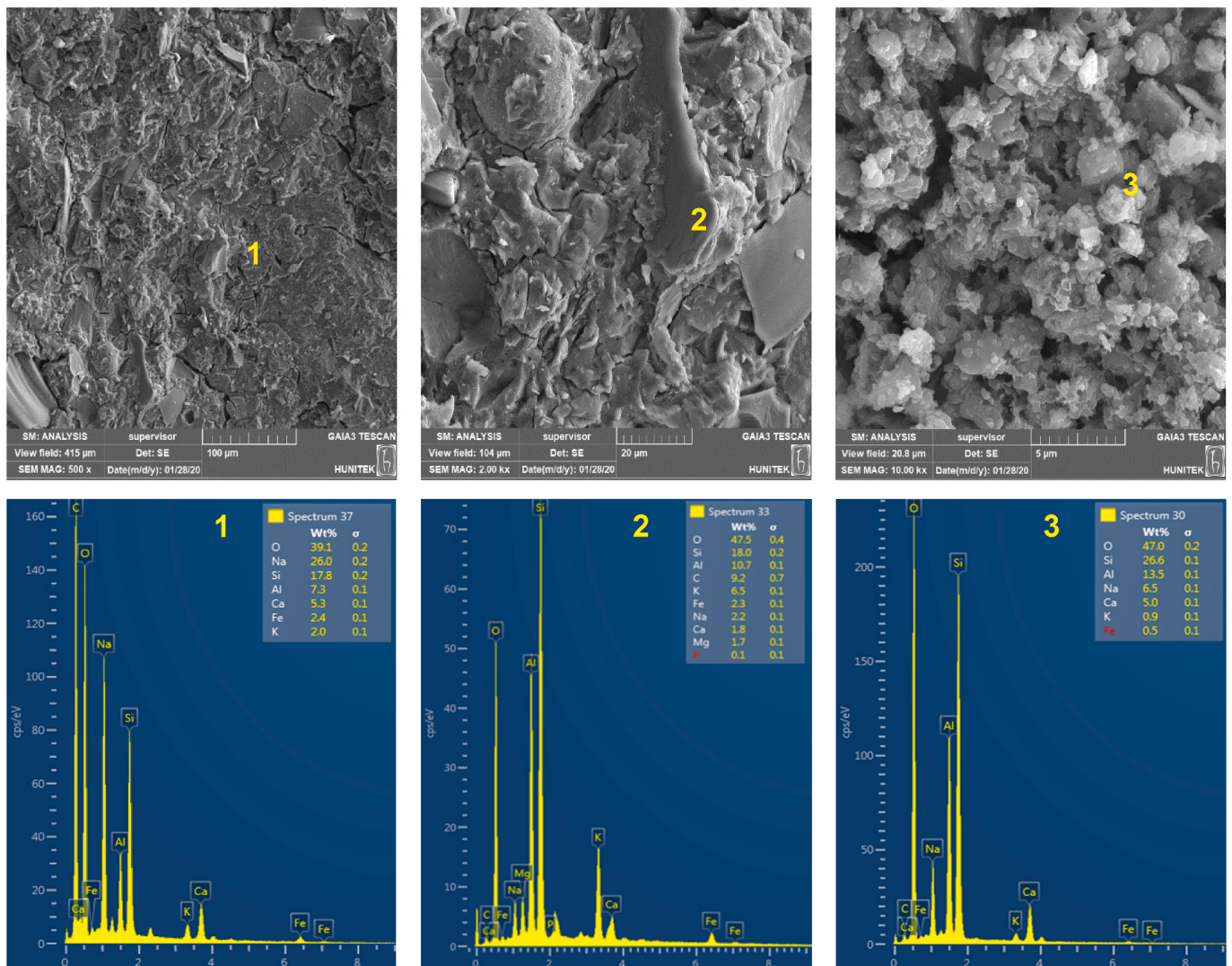
Fig. 8. SEM micrographs with EDX spectra of 25RCB-75RT alkali-activated binder activated with 15 M NaOH solution and cured at 115 °C for 48 h.
