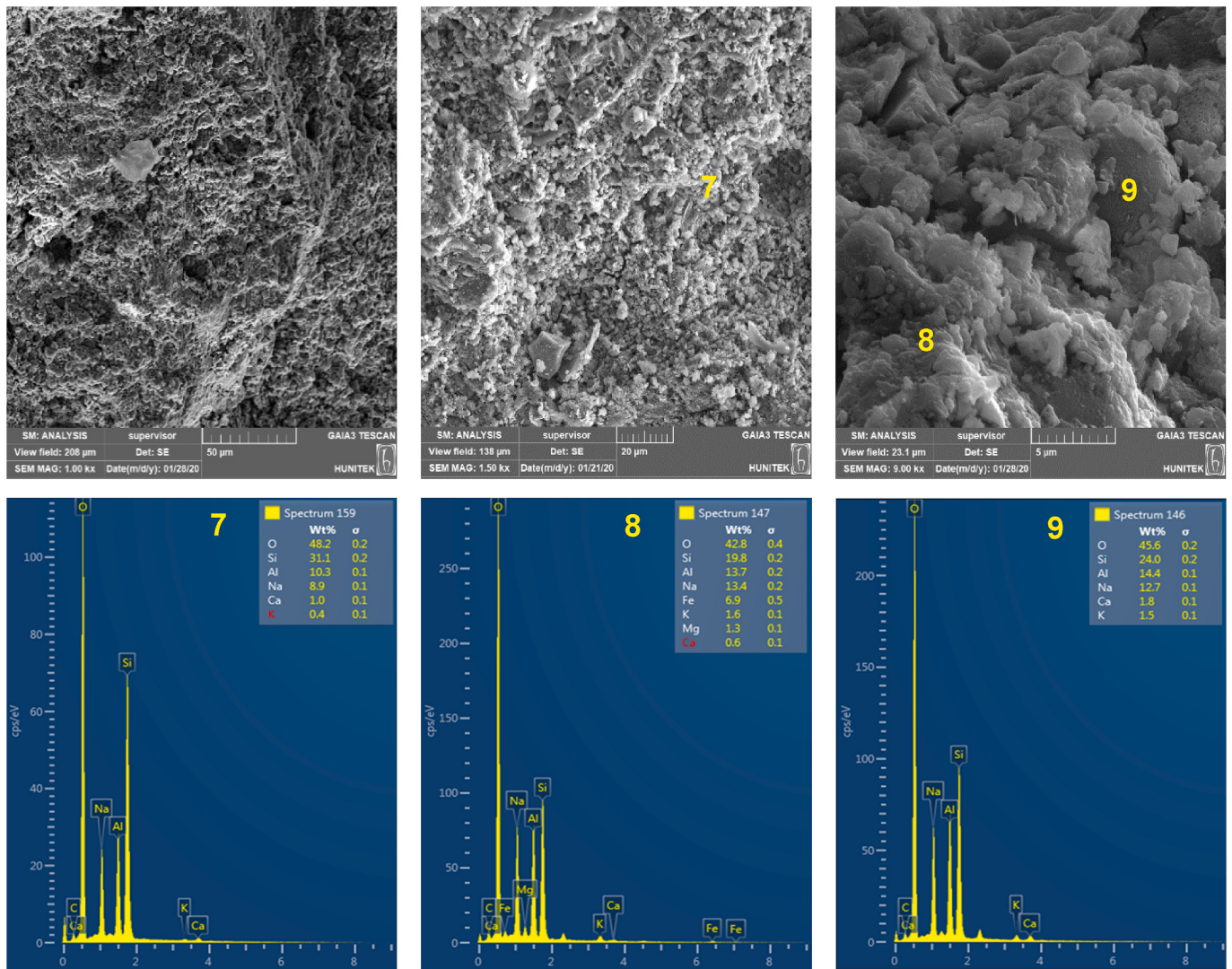
Fig. 10. SEM micrographs with EDX spectra of 25RT-75HB alkali-activated binder activated with 15 M NaOH solution and cured at 115 °C for 48 h.
