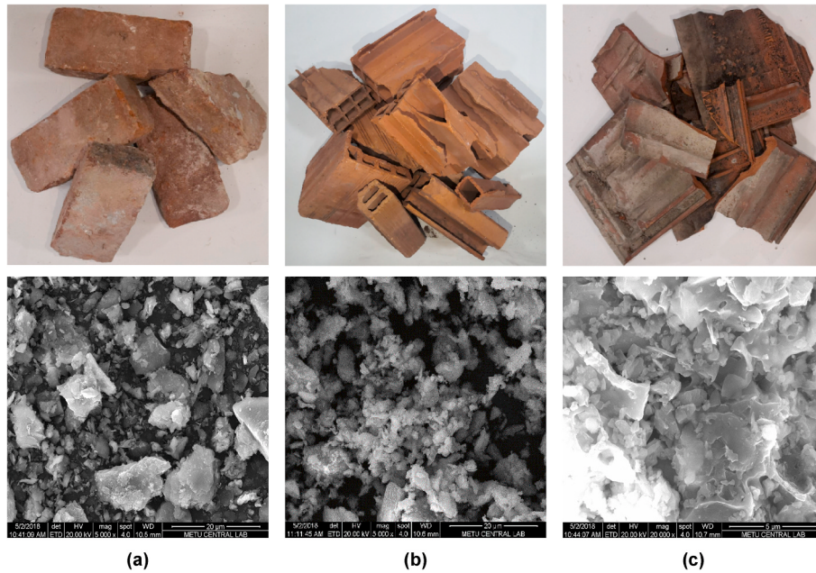
Fig. 1. Video camera and SEM views of CDW-based precursors (a) red clay brick (RCB), (b) hollow brick (HB), (c) roof tile (RT).
