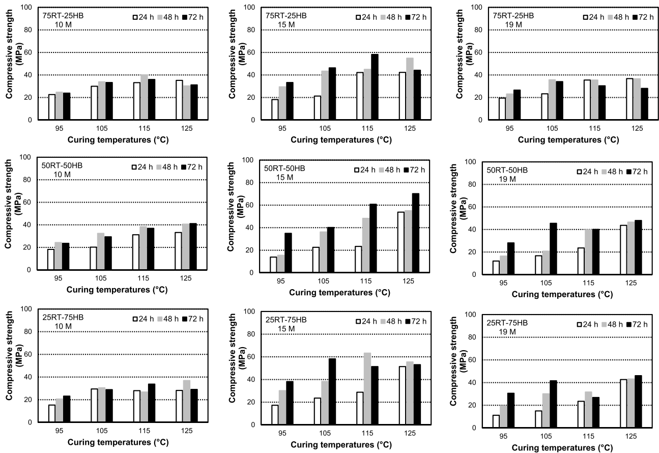
Fig. 6. Average compressive strength results of alkali-activated binders with different substitution rates of RT and HB.
