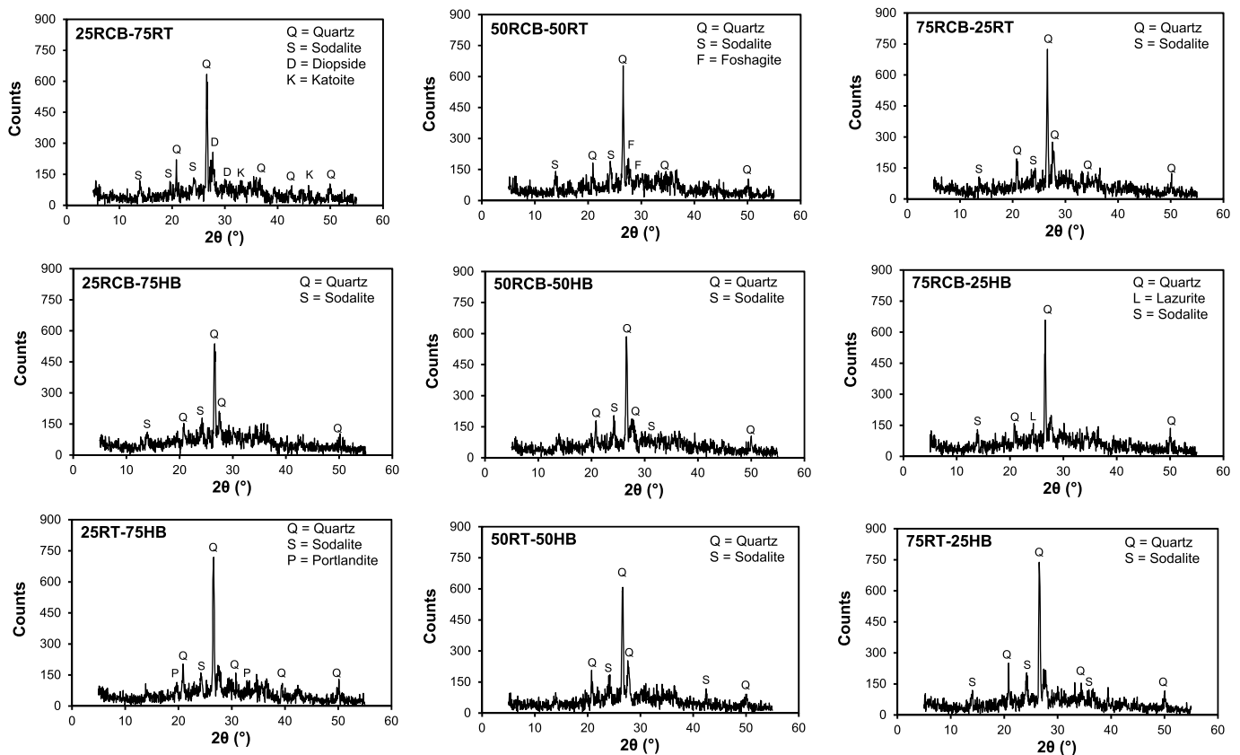
Fig. 7. XRD diffractograms of alkali-activated binders having different substitution rates of CDW-based precursors, activated with 15 M NaOH solution and cured at 115 °C for 48 h [Quartz ( \text{SiO}_2 ) PDF No: 96-101-1160, Sodalite ( \text{Na}_4\text{Al}_3\text{Si}_3\text{O}_{12}\text{Cl} ) PDF No: 96-900-3326, Diopside ( \text{CaMg}_{0.7}\text{Si}_{1.7}\text{O}_6 ) PDF No: 96-900-5280, Katoite ( \text{Ca}_3\text{Al}_2\text{Si}_3\text{O}_{12}\text{H}_{12} ) PDF No: 96-900-2709, Foshagite ( \text{Ca}_4\text{Si}_3\text{O}_{11}\text{H}_2 ) PDF No: 96-901-1044, Lazurite ( \text{Na}_{3.48}\text{Ca}_{0.6}\text{Al}_{2.91}\text{Si}_{3.09}\text{O}_{11.52}\text{S} ) PDF No: 96-901-1357, Portlandite ( \text{Ca}(\text{OH})_2 ) PDF No: 96-900-6836].
