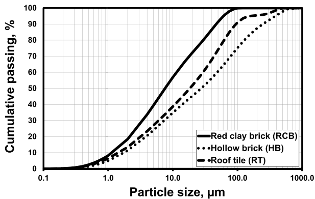
Fig. 2. Gradation curves of CDW-based precursors.
