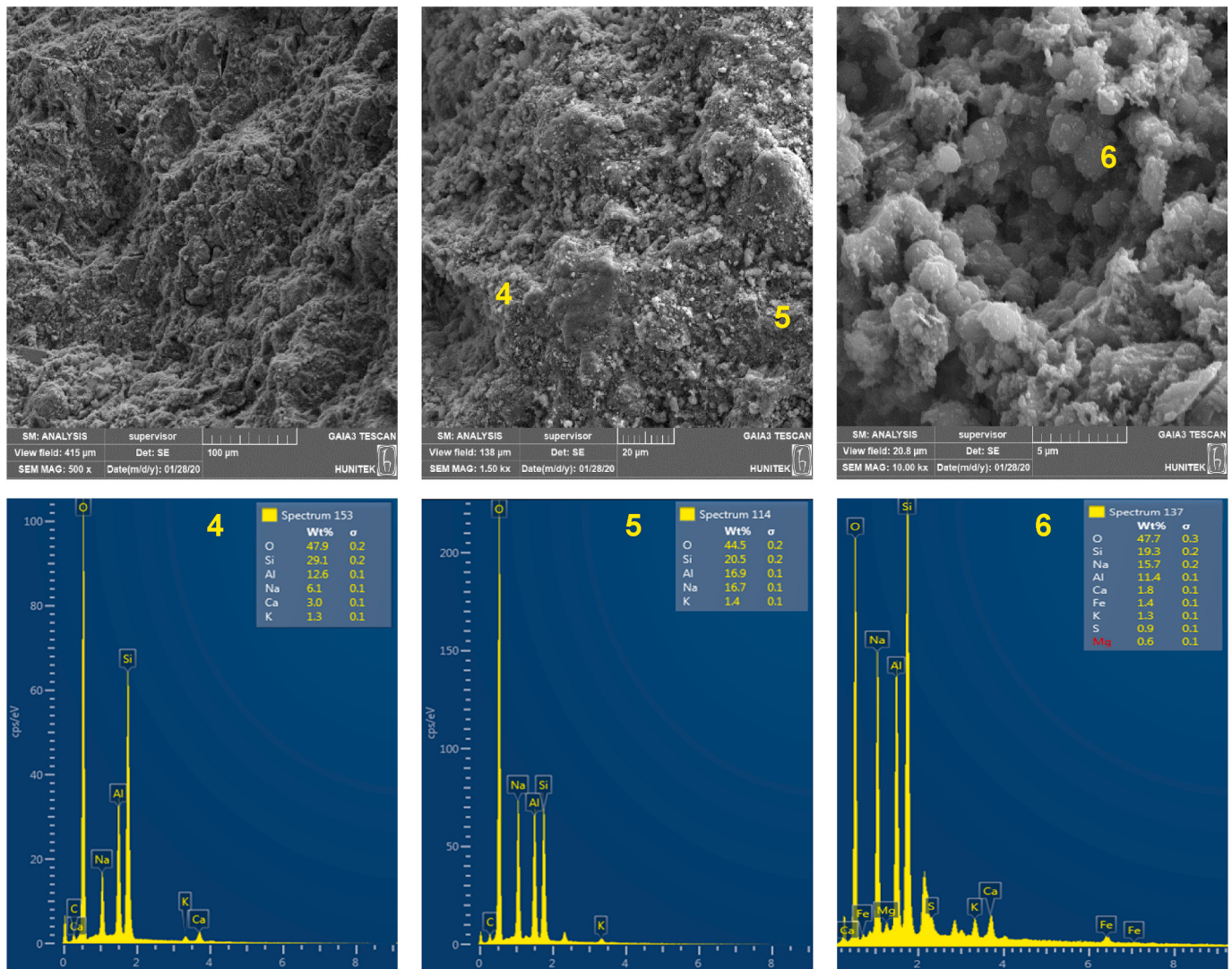
Fig. 9. SEM micrographs with EDX spectra of 25RCB-75HB alkali-activated binder activated with 15 M NaOH solution and cured at 115 °C for 48 h.
