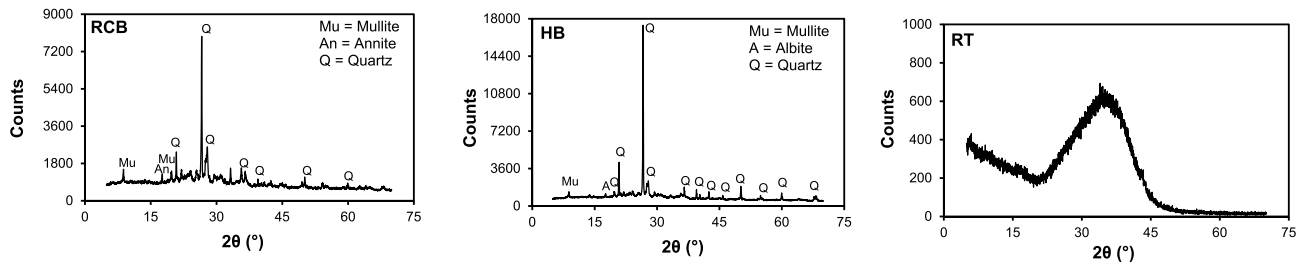
Fig. 3. XRD diffractograms of CDW-based precursors (Particle diffraction file [PDF] numbers: Mullite ( \text{Al}_2\text{Si}_0.7\text{O}_{4.8} ) PDF No: 96-900-1568, Albite ( \text{NaAlSi}_3\text{O}_8 ) PDF No: 96-900-2201, Annite ( \text{K}_{0.94}\text{Fe}_{2.43}\text{Al}_{2.15}\text{Si}_{2.43}\text{O}_{12} ) PDF No: 96-900-2310, Quartz ( \text{SiO}_2 ) PDF No: 96-101-1160).
