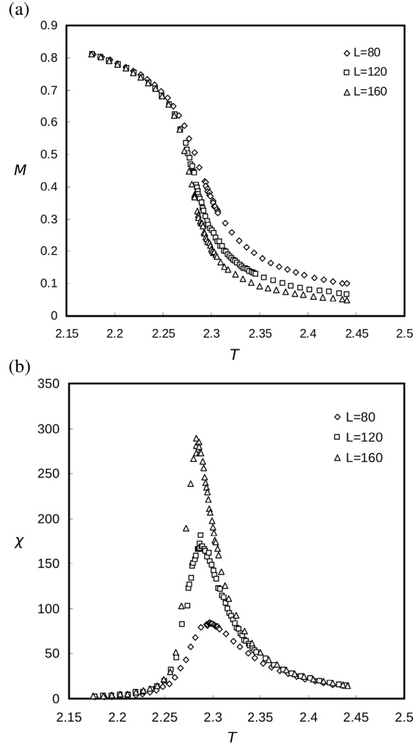
Fig. 3. Temperature dependence of (a) the order parameter ( M ) and (b) the magnetic susceptibility ( \chi ) of the two-dimensional Ising model for the lattice with L = 80 , 120, and 160.
