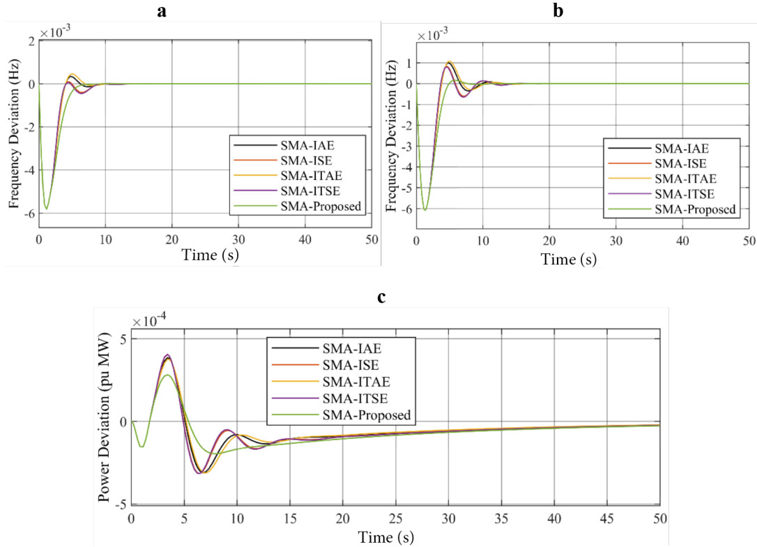
Figure 7. Deviations; a) frequency of area-1, b) frequency of area-2, c) power of tie-line.
