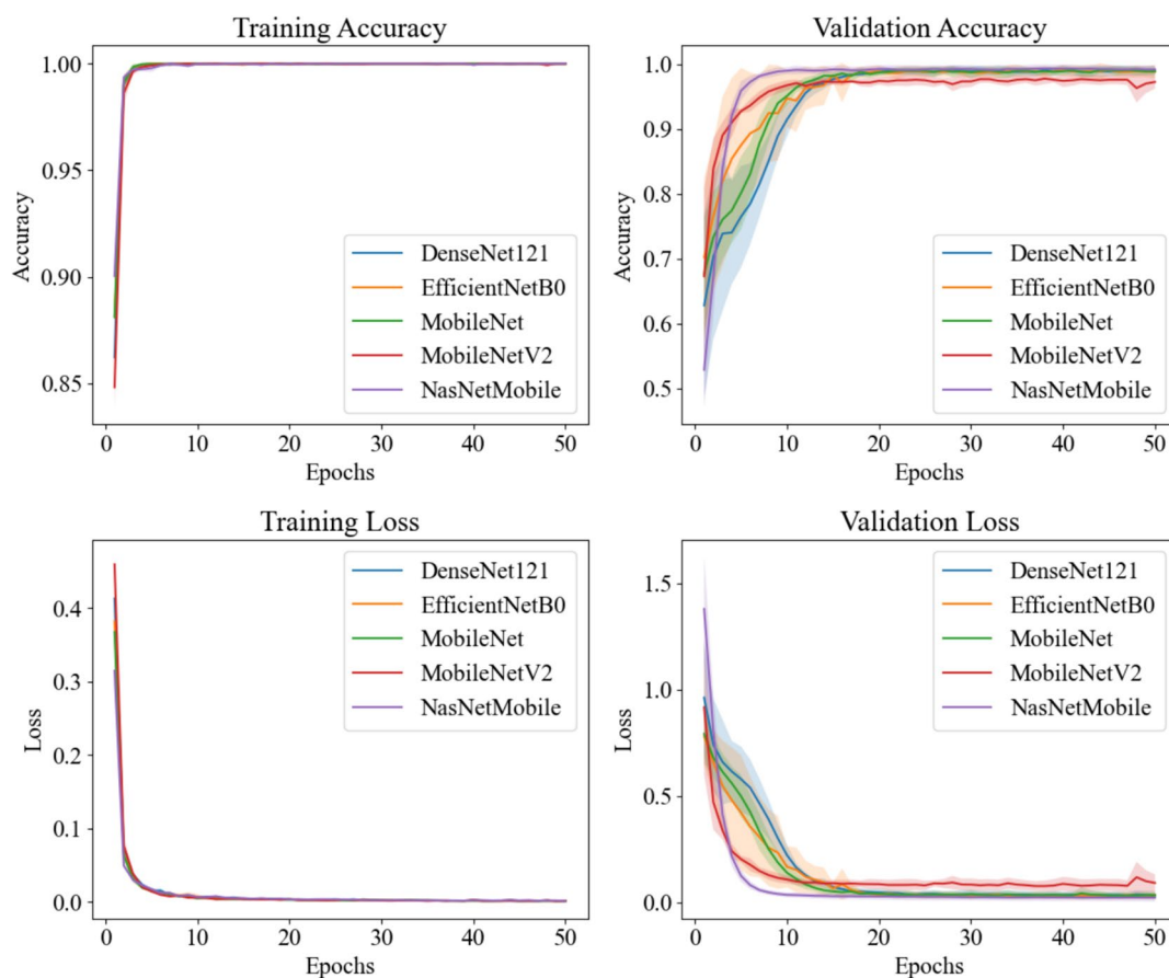
Fig 9 The mini-batch accuracy and loss graphs of the CNN models
