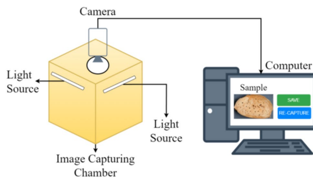
Fig. 1 Data collection system
