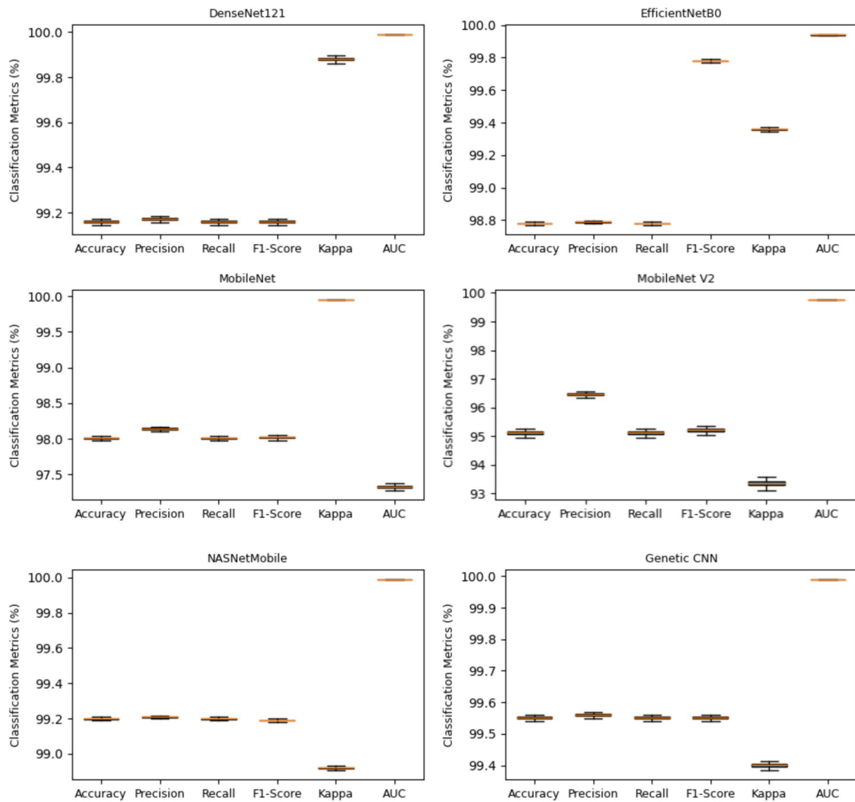
Fig. 12 Box plot diagrams illustrating the classification metrics of cnn models
