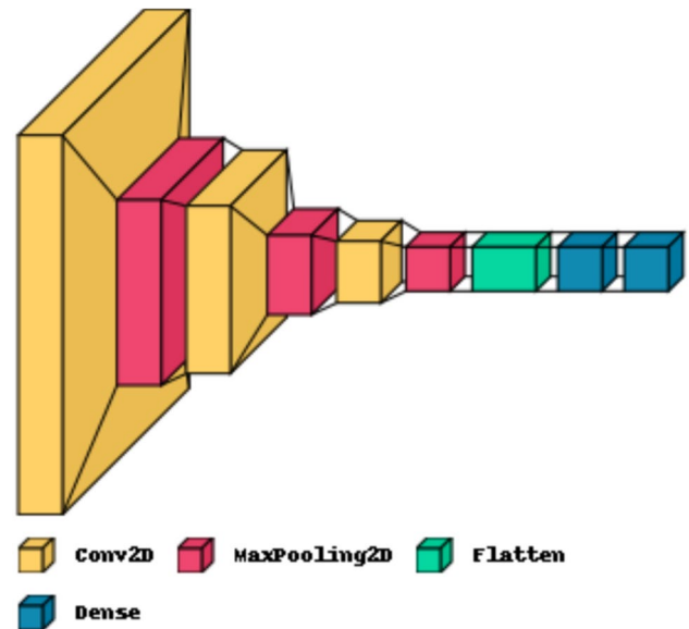
Fig. 4 Genetic CNN architecture
