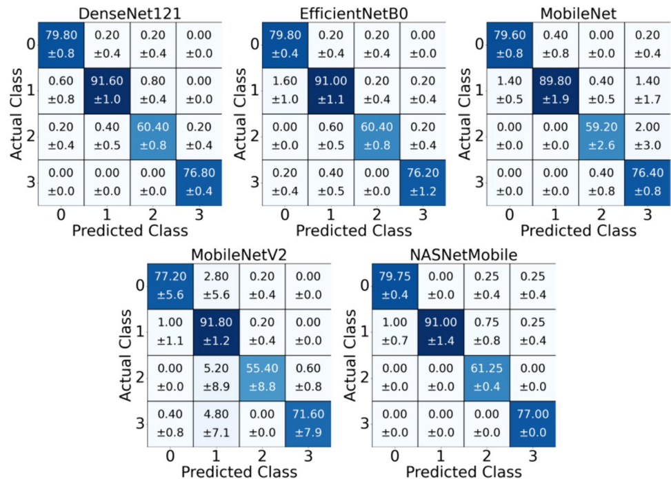
Fig. 8 Confusion Matrices of CNN models (0: Ak, 1: Kapadokya, 2: Nurlu, 3: Sira)
