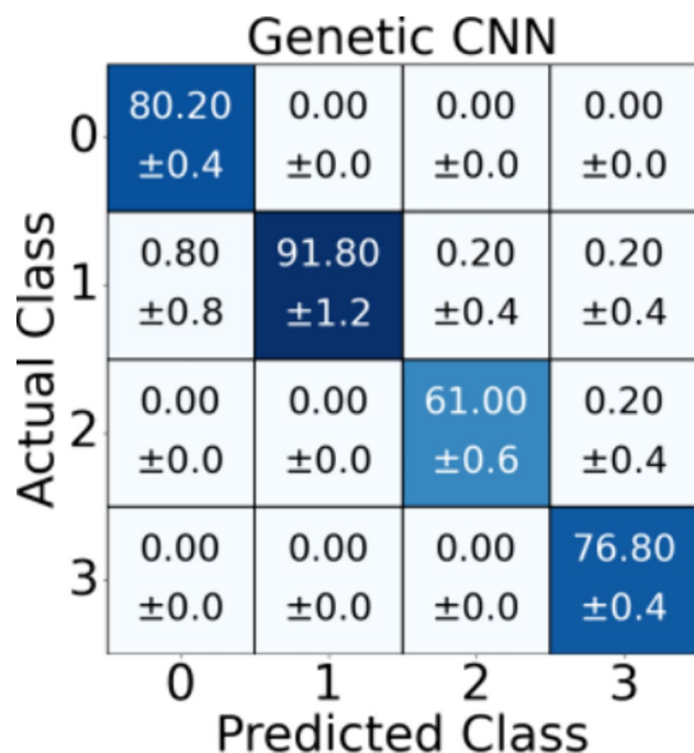
Fig. 10 Confusion matrix of Genetic CNN (0: Ak, 1: Kapadokya, 2: Nurlu, 3: Sira)
