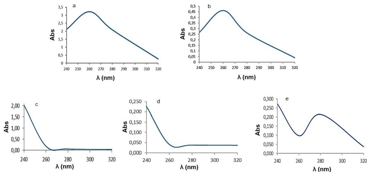
Fig. 1 – UV-absorbance spectra of the tested molecules (a – ct-DNA, b – S. aureus DNA, c – Melamine 10 mM, d – Cyanuric acid 15 mM, e – Uric acid 1 mM).
