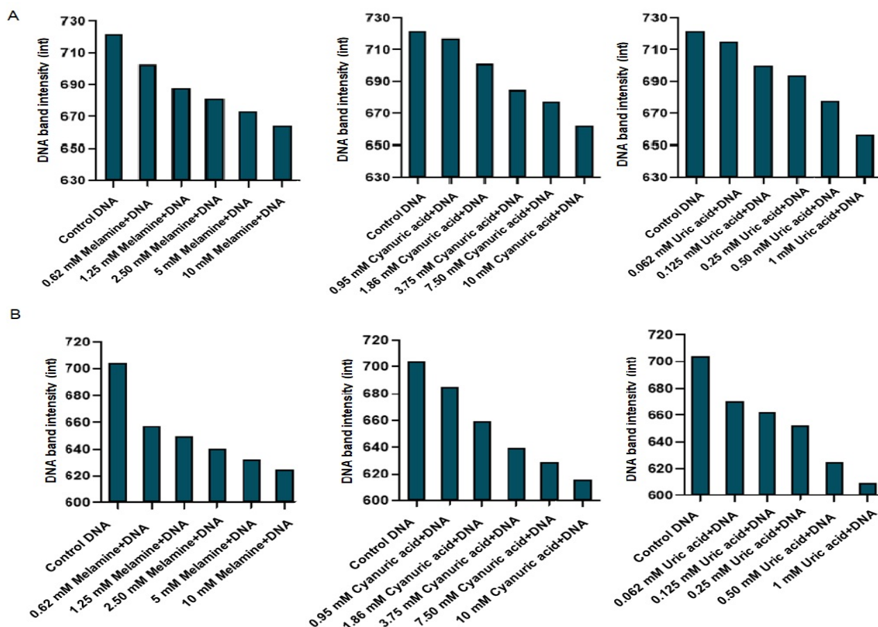
Fig. 5 – DNA band intensities obtained from images of agarose gel electrophoresis. A: Calf thymus genomic DNA+melamine/metabolites, B: S. aureus DNA+melamine/metabolites.
