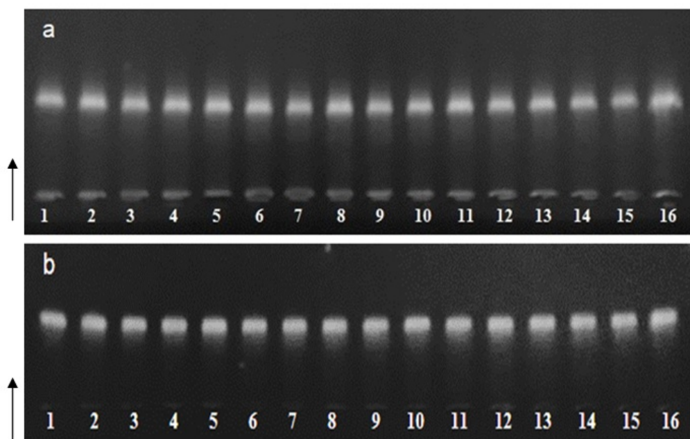
Fig. 4 – DNA+melamine/metabolites agarose gel images: (a) ct-DNA and (b) S. aureus DNA. Lanes 1,2,3,4 and 5 exhibit DNA+melamine (0.62, 1.25, 2.50, 5, 10 mM), lanes 6,7,8,9 and 10 show DNA+cyanuric acid (0.95, 1.86, 3.75, 7.50, 15 mM), lanes 11,12,13,14 and 15 indicate DNA+uric acid (0.062, 0.125, 0.25, 0.50, 1 mM), lane 16 is the control DNA. Arrows indicate the direction of DNA migration in agarose gel.
