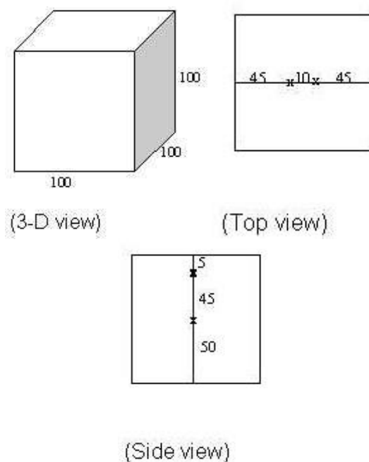
Fig. 3. The location of the thermocouples in the concrete cube specimens (the dimensions are given in cm)
