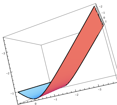
Figure 4. Cylindrical surface x(s, t) over binormal B(s) of pseudo null curve
