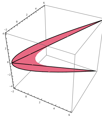
Figure 1. Tangent surface \phi(s, t) over the pseudo null circle
