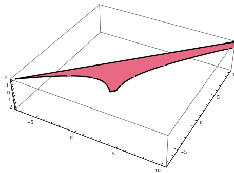
Figure 3. Principal normal surface \phi(s, t) over the pseudo null helix
