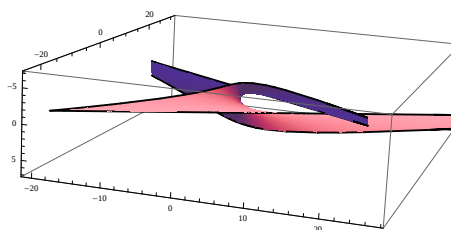
Figure 2. Binormal surface \phi(s, t) over the pseudo null helix
