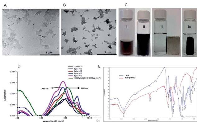
Fig. 2 (A) TEM image of bare GO, (B) TEM image of mGO, (C) photograph of (i) GO, (ii) mGO, (iii), mGO with a magnet, and (iv) mGO collected on glass vial. (D) UV-vis spectra of ICG and ICG@mGO; (E) FTIR spectra of ICG and ICG@mGO.
