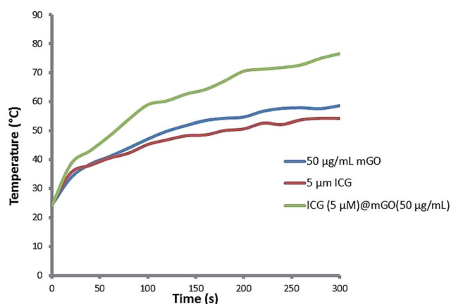
Fig. 4 Heat generation produced by mGO, ICG and ICG@mGO.
